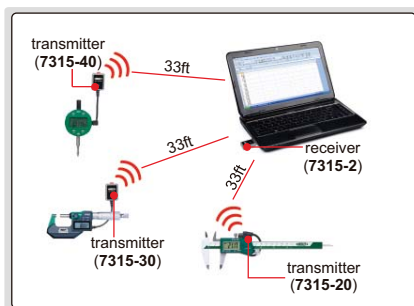
7315-2 application (multichannel)
