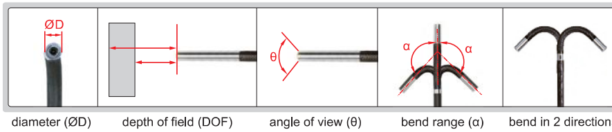
diameter (ØD) depth of field (DOF) angle of view ( \theta ) bend range ( \alpha ) bend in 2 directions
