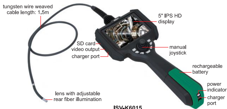
ISV-K6015
